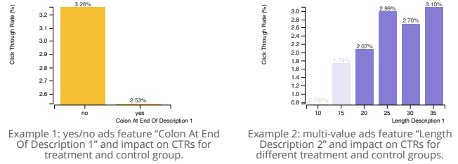
Figure 2: Bi- and multipolar ad features with CTRs
